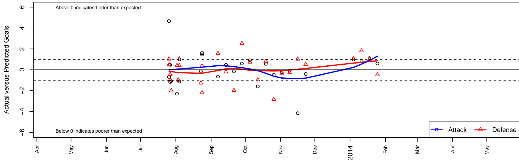
BIFC Blue B02 Dots are actual minus expected GF (blue circles) and GA (red triangles). Blue line is smoothed change in attack strength. Red is smoothed change in defense strength.
